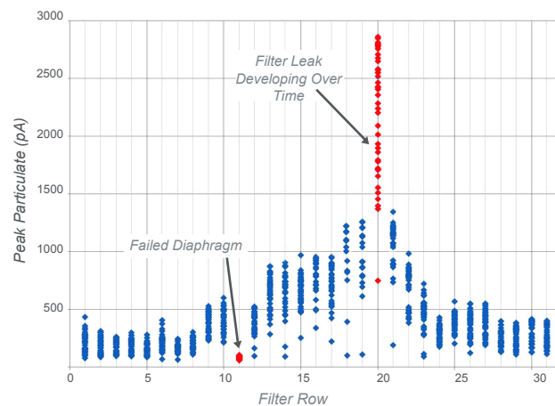
Figure 1: Particulate values over 39 pulse cycles confirm developing leak (row 20). While diaphragm failure is principally detected by pressure signal analysis, it is also detectable here (row 11).
