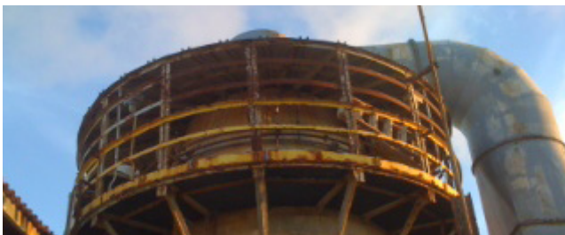
Acid discharge caused by baghouse upset conditions resulted in damage to process equipment structure.
