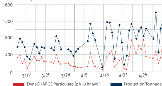
Figure 2 -- Relative Mass Emissions vs Production Rates
